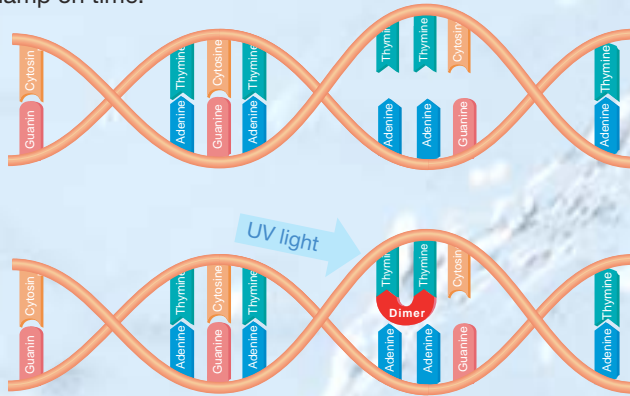
UV Destroys Microorganisms by Disrupting Their DNA
