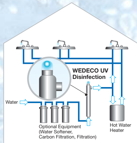
Typical WEDECO UV Installation
